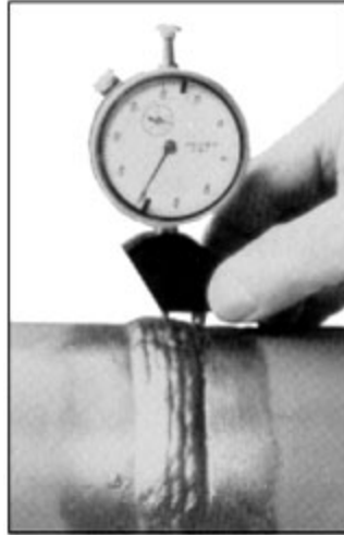
Measures Undercut Butt Weld
