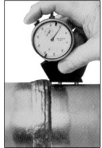
Measures Crown Height Butt Weld
