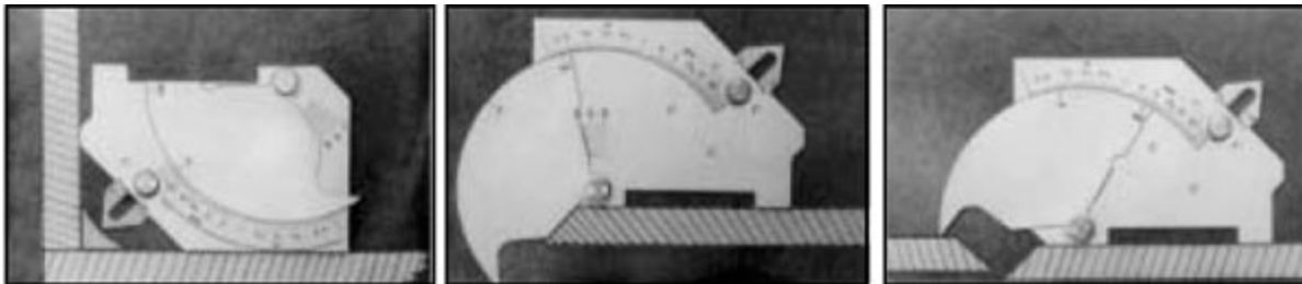
FILLET WELD THROAT
