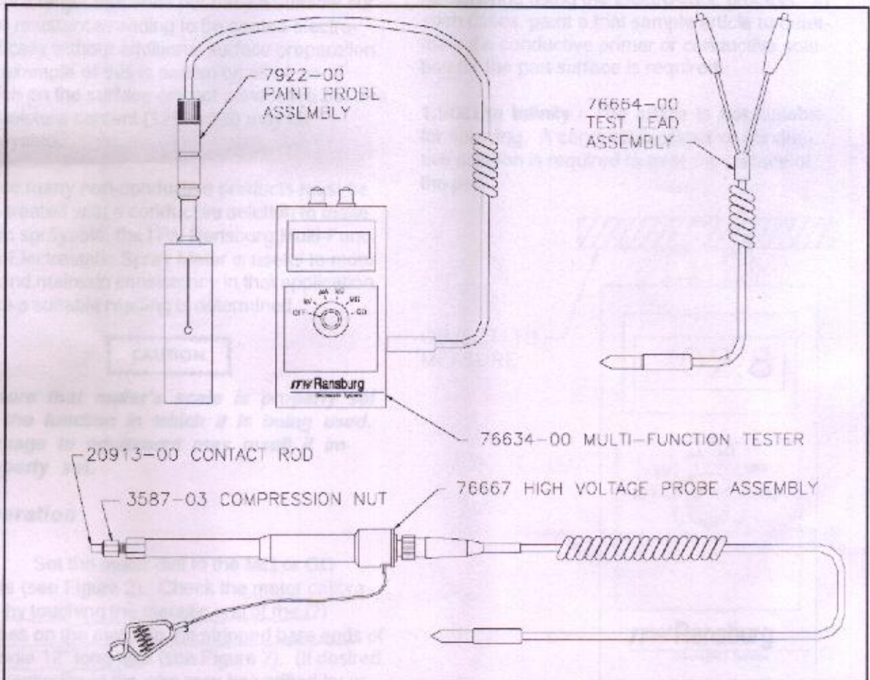
Figure 1B: Multi-Function Meter Kit Parts
